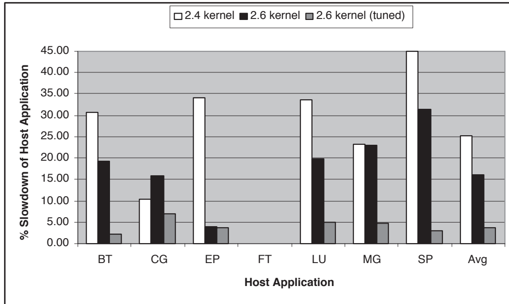
Fig. 3. Comparison of slowdown of the host application in shared mode when run on different kernels
