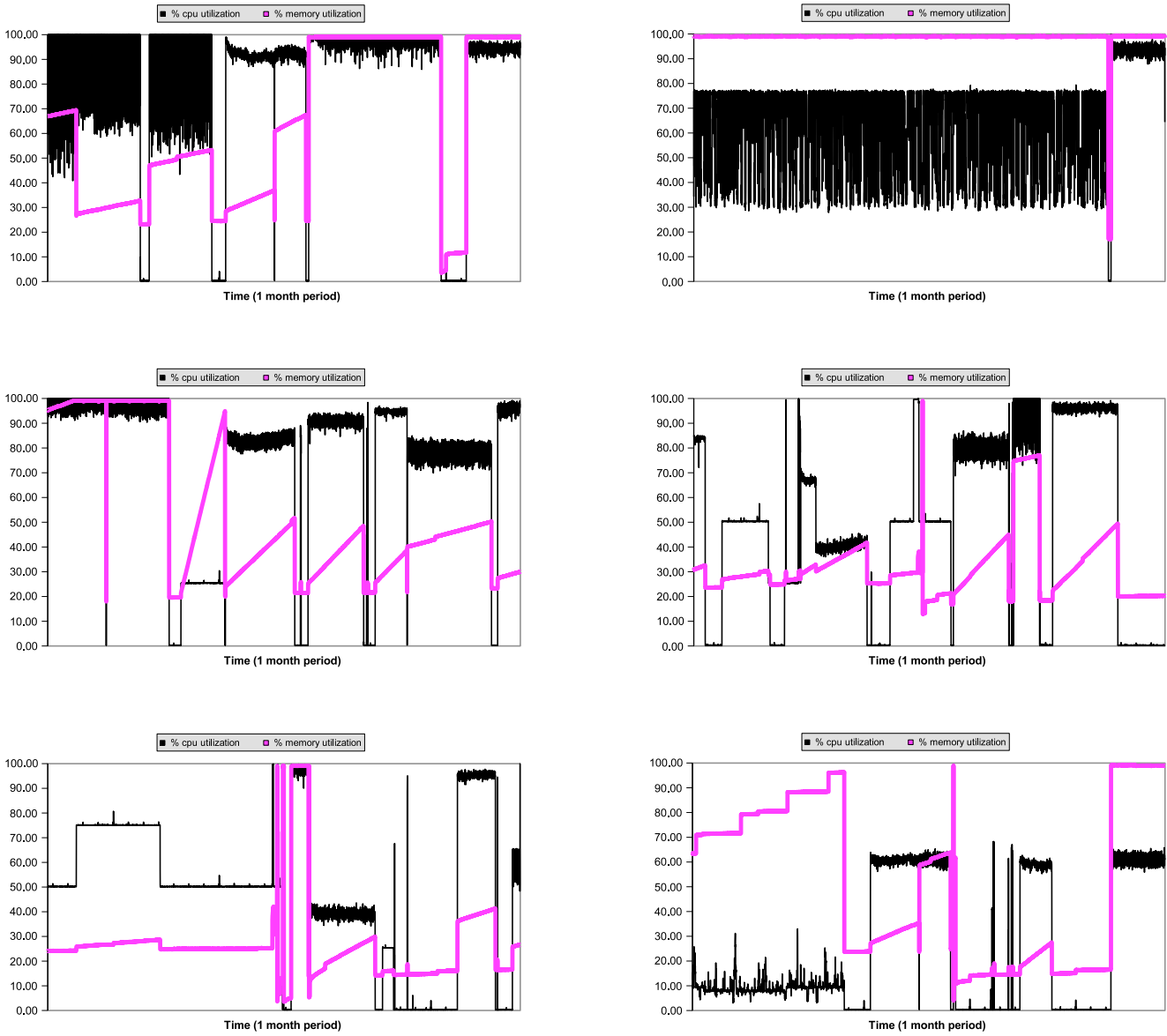
Fig. 1. CPU and Memory utilization of nodes of a busy cluster plotted over a period of 1 month
