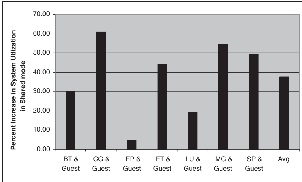
Fig. 5. Percent increase in efficiency of the system for different benchmarks
