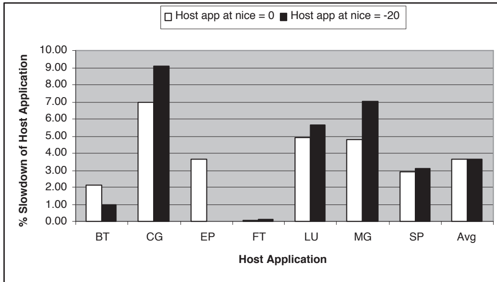
Fig. 4. Comparison of percent slowdown of the host application when running at normal priority (nice = 0) vs. when running at highest priority (nice = -20) in shared mode
